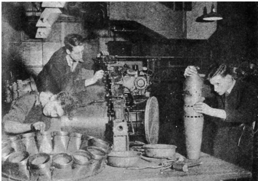
Assembling combustion details on Goblin. Mick Goode on right with flame can.
